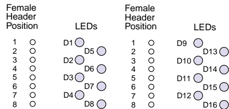
Figure 3. LED Positions
