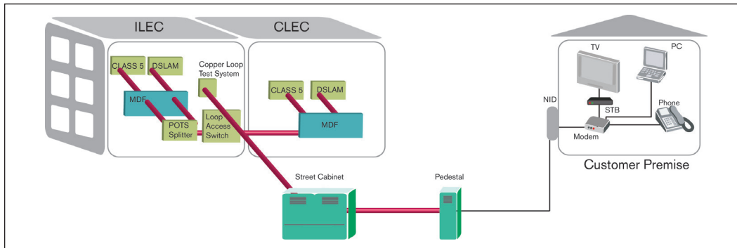
Test from CO to Subscriber
