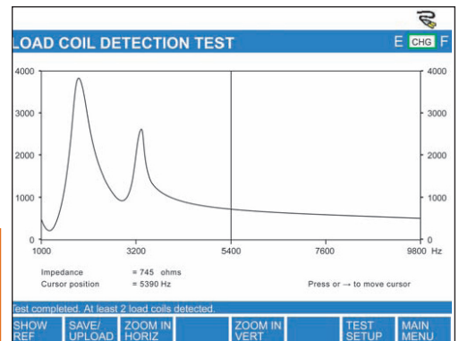
Easily Detect Number of Load Coils Deployed
