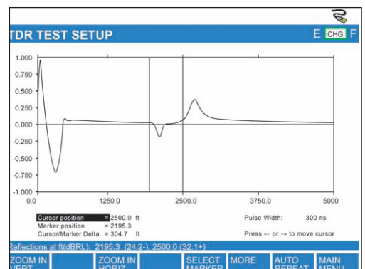
4 Wire TDR Test Result
