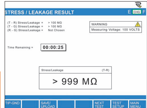
Stress/Leakage Test
